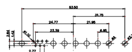
13W6 Female
