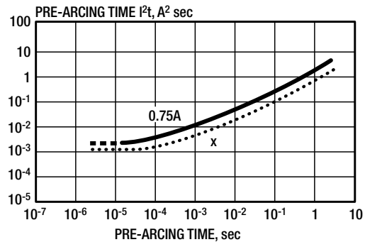
Fig. 6b. Choice of 0.75A fuse, example #6. ----- Pre-arcing I²t ----- Maximum I²t design rule x I²t for sample current pulse
