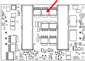
Figure 15. Temperature Monitoring Locations
