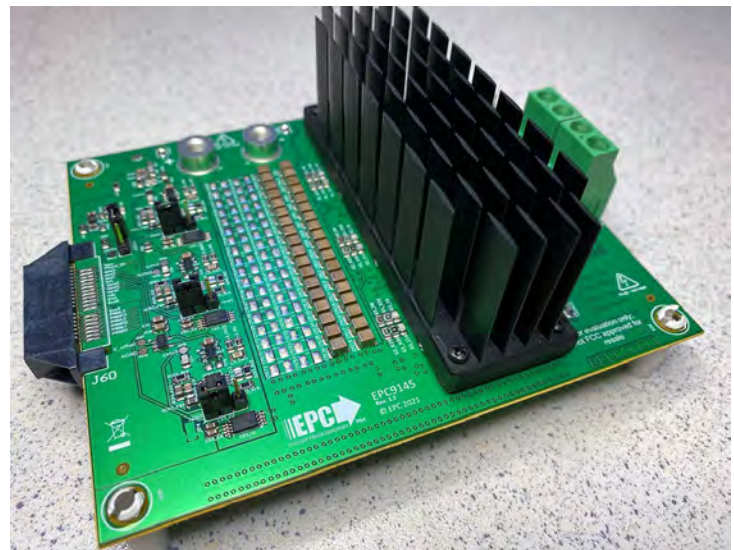
EPC9145 Demonstration board with heatsink attached
