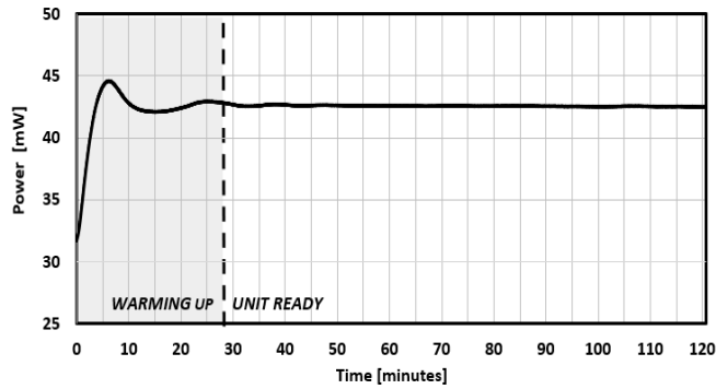
FIG. 15: WARM-UP TIME
