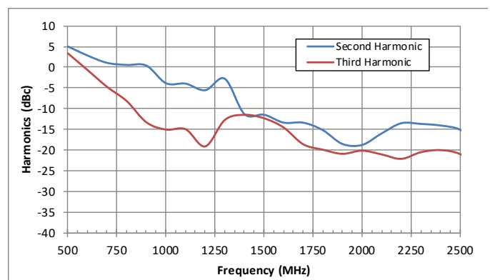
Harmonics (@ Psat)
