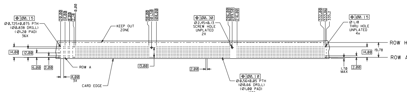
DAUGHTERCARD HOLE PATTERN (CONNECTOR SIDE)
