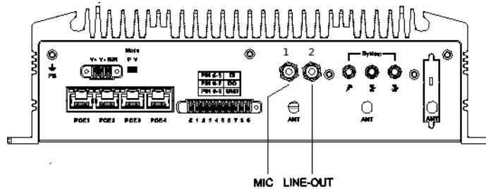
Figure 4.22 Cellular Voice Connector
