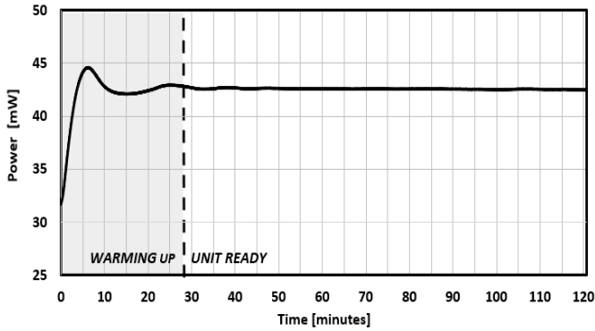
FIG. 15: WARM-UP TIME
