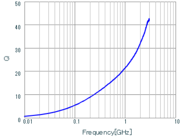
LQP02TQ2N7C02 Q.
