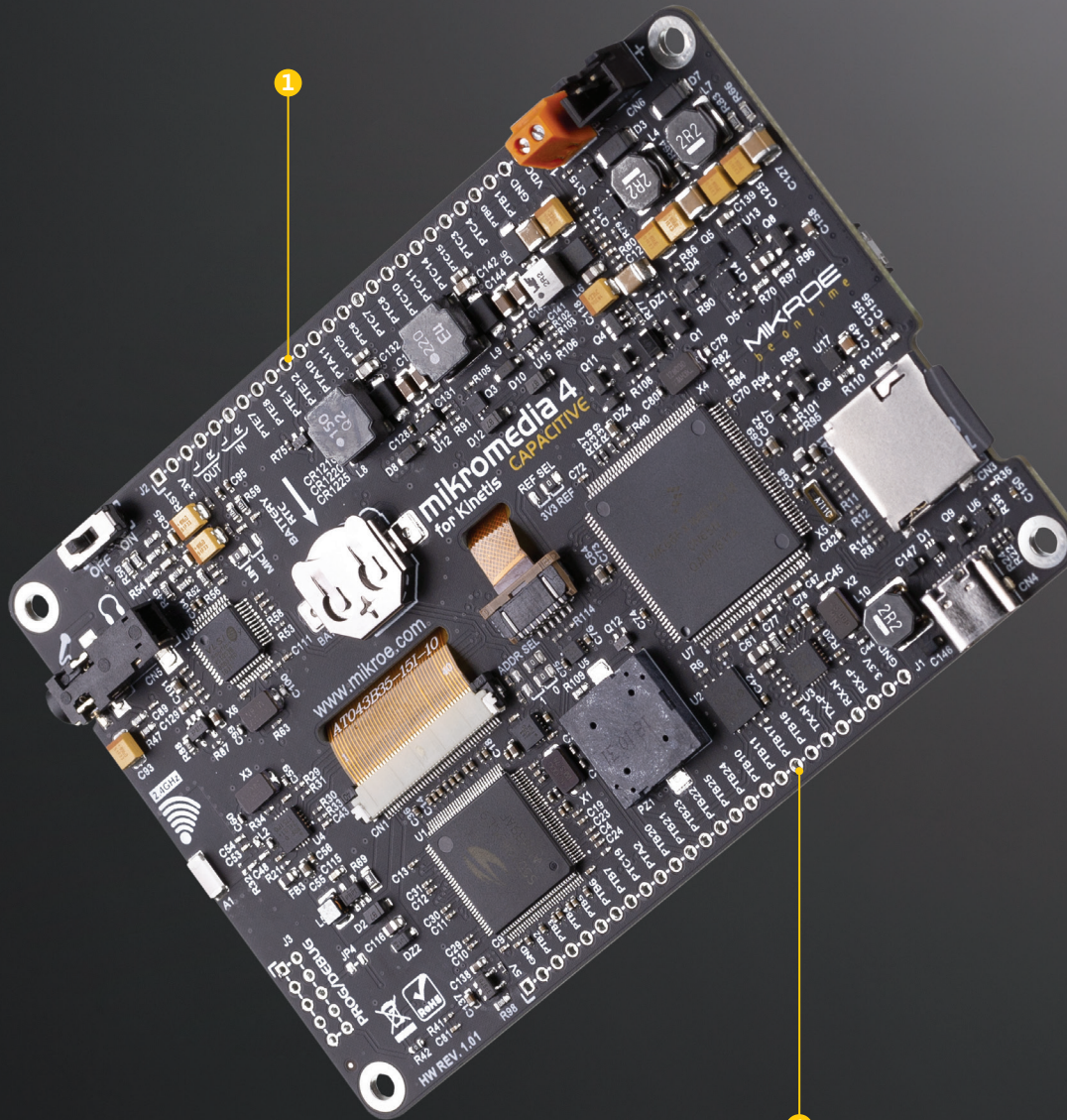
Figure 14: mikromedia 4 back view
