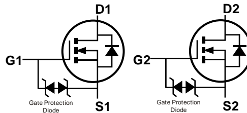
Internal Schematic
