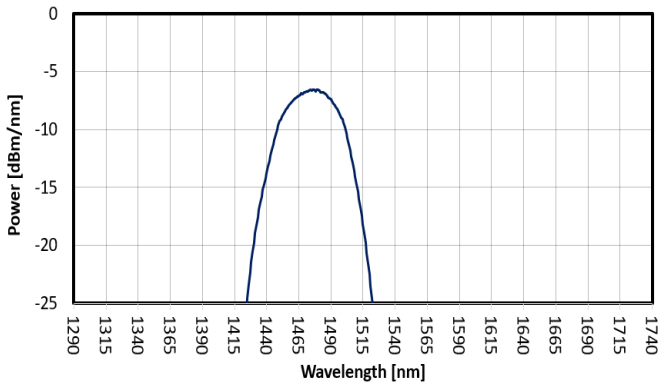
FIG. 5: SLED 4 SPECTRUM
