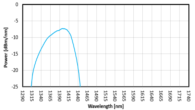
FIG. 6: SLED 5 SPECTRUM
