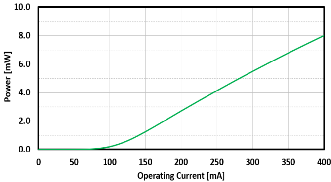
FIG. 7: SLED 1 OUTPUT POWER VS CURRENT
