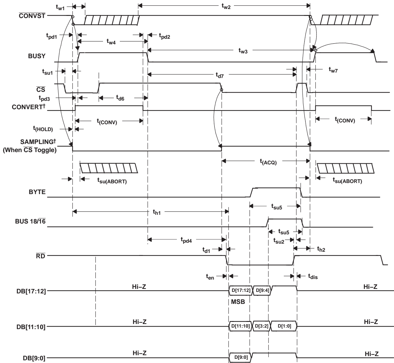
Figure 30. Timing for Conversion and Acquisition Cycles With \overline{\text{CS}} and \overline{\text{RD}} Toggling
