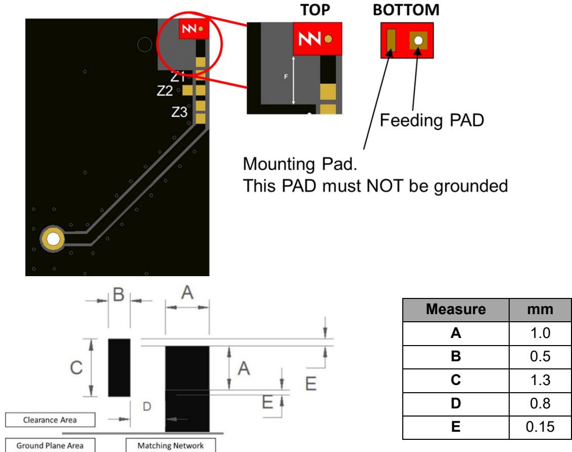
Figure 8 - Footprint dimensions for the NANO mXTEND™ (NN02-101) antenna booster (on the corner).
