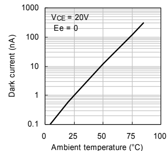
Dark Current vs. Ambient Temperature
