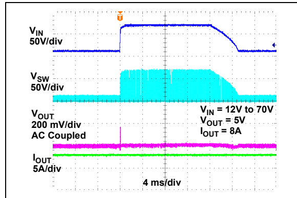
FIGURE 2-68: Line Transient Response ( V_{IN} = 12V\text{ to }70V ).
