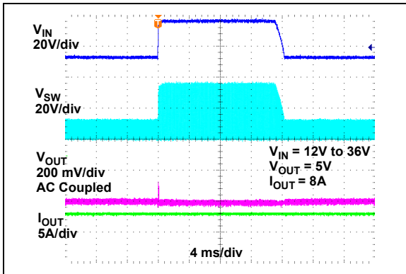
FIGURE 2-66: Line Transient Response ( V_{IN} = 12V\text{ to }36V ).
