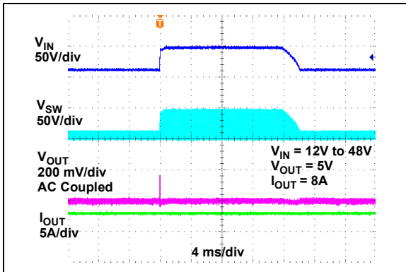
FIGURE 2-67: Line Transient Response ( V_{IN} = 12V\text{ to }48V ).
