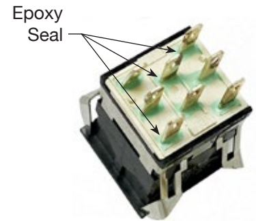
An Example of Epoxy Seal at Base of Terminals Before the Change
