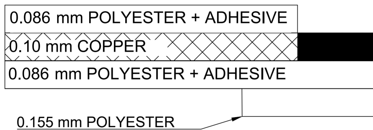
CROSS-SECTION
