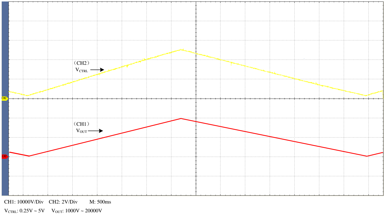
Figure 3. Triangle Wave
