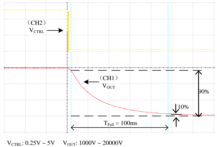
Figure 7. Fall Time
