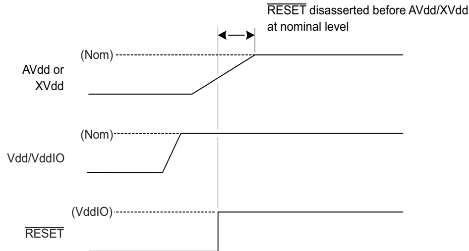
Figure 7-2. Power Sequencing on the mXT2952T2 – Late rise on AVDD or XVdd
