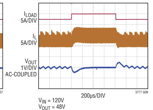
Load Step Buck Region Pulse-Skipping Mode
