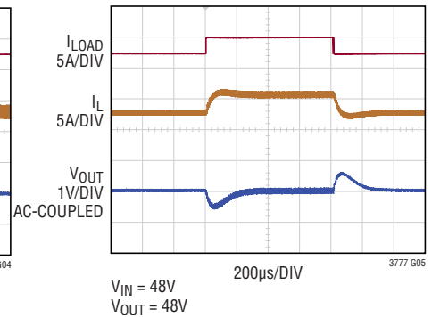
Load Step Buck-Boost Region Continuous Mode
