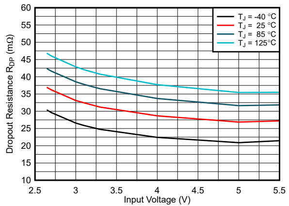
Figure 7-4. Dropout Resistance
