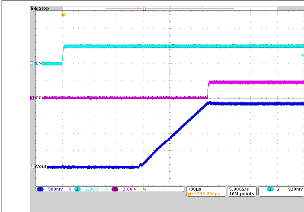
Figure 9-20. Start-Up Timing
