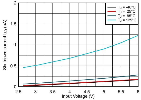
Figure 7-2. Shutdown Current
