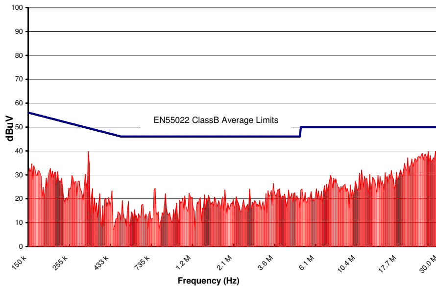
Figure 18. CPE4D18 Conducted Emissions using above specified input filter, Vin = 24V, Full Resistive Load
