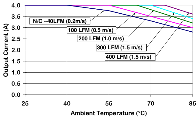
Figure 3. Output Current Derating vs Ambient Temperature & Airflow (air flowing from pin 3 to to pin 1, Vin = 12 V without baseplate)
