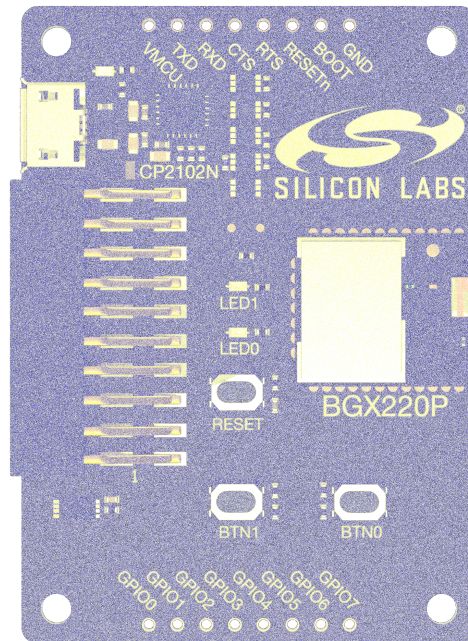
Figure 1.1. BGX220P Expansion Board
