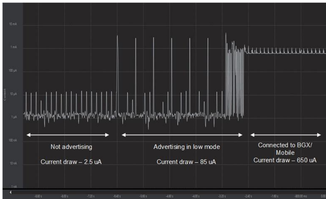
Figure 4.3. Energy Profiler Capture of BGX13 with 9600 bps UART Baud Rate
