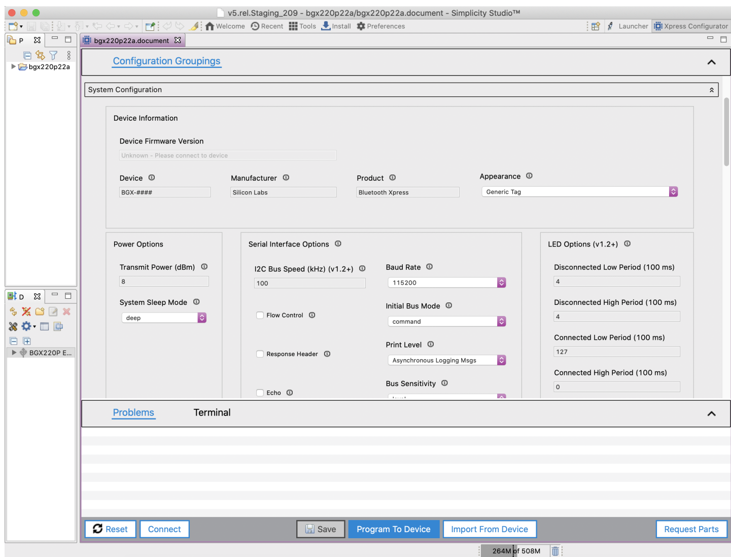
Figure 2.1. Xpress Configurator
