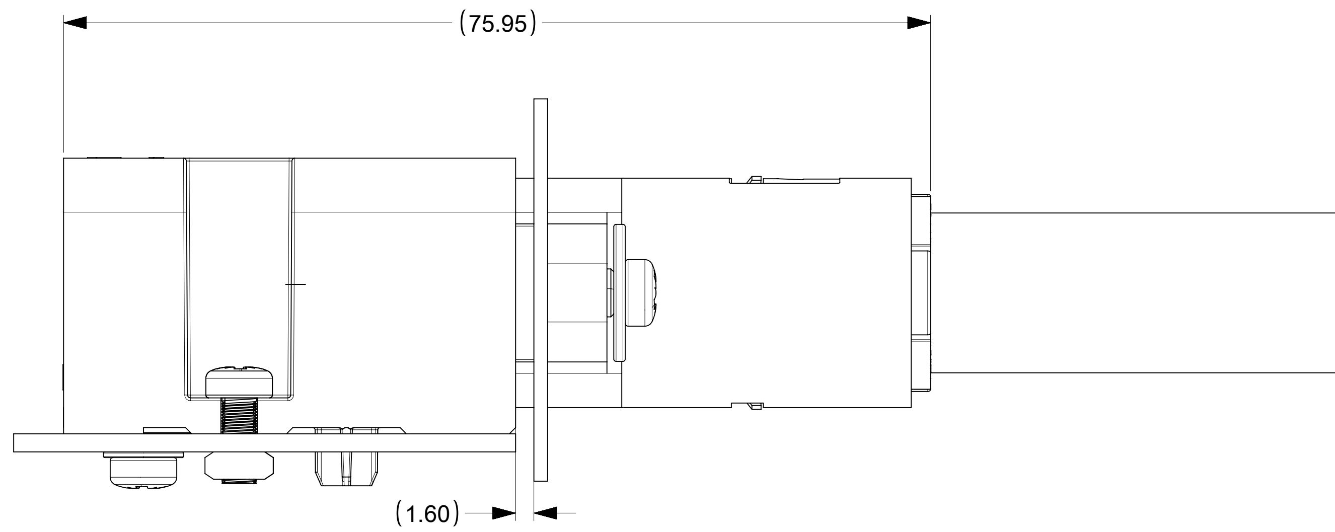
ASSEMBLED AND MATED WITH RA HEADER_SCREW MOUNT VERSION (2155108031)
