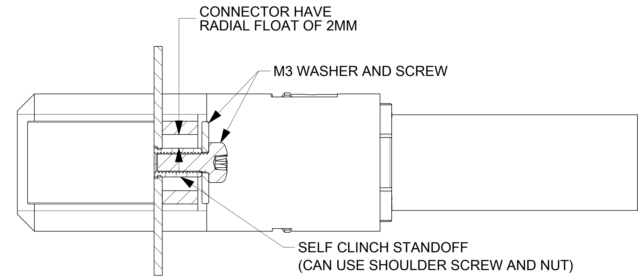
SECTION B-B
