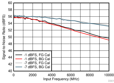
JMODE 3, f_s = 3200 \text{ MHz} , foreground (FG) and background (BG) calibration
