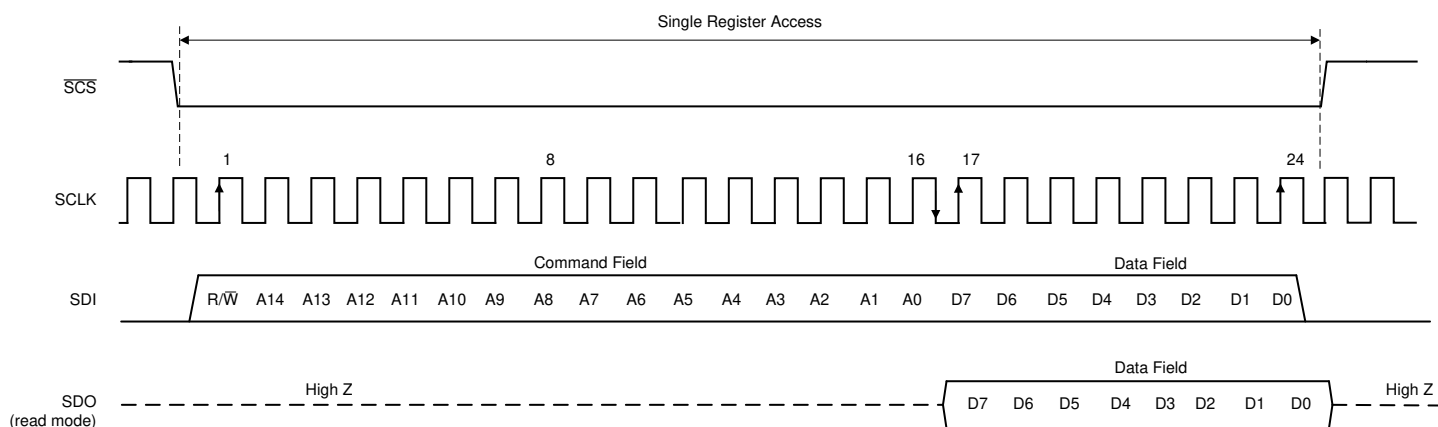
Figure 7-24. Serial Interface Protocol: Single Read/Write
