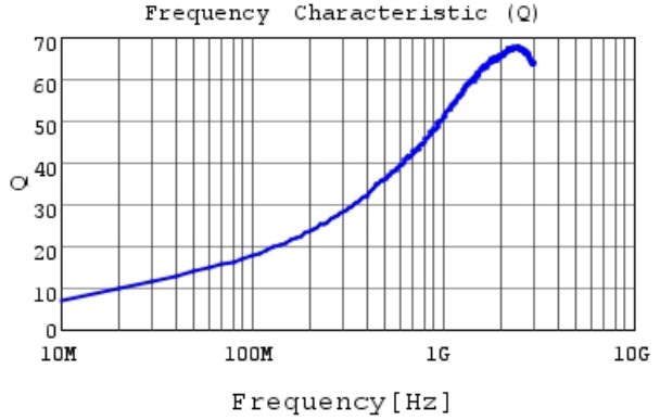
LQG15WZ4N1B02 Q
