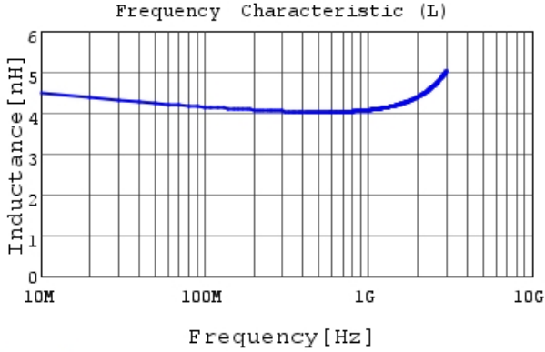
LQG15WZ4N1B02 L
