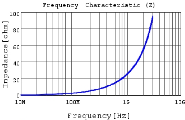
LQG15WZ4N1B02 |Z|
