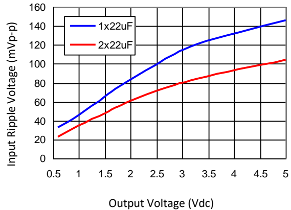
Figure 46. Input ripple voltage for various output voltages with 1x22 µF or 2x22 µF ceramic capacitors at the input (6A load). Input voltage is 12V.
