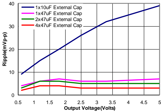
Figure 47. Output ripple voltage for various output voltages with external 1x10 μF, 1x47 μF, 2x47 μF or 4x47 μF ceramic capacitors at the output (6A load). Input voltage is 12V.
