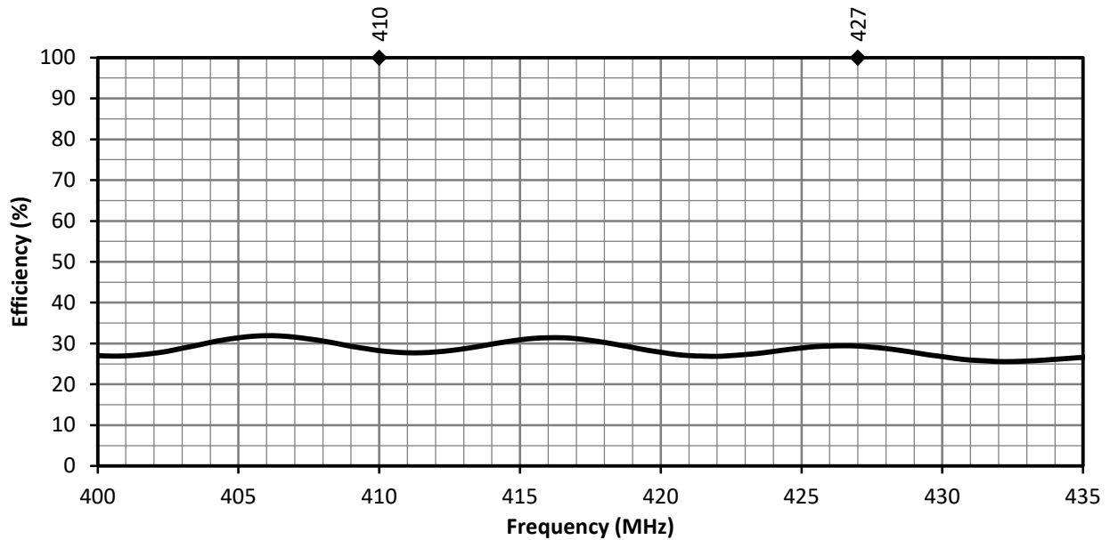
Figure 9. ANT-410-WRT Antenna Radiation Efficiency, Free Space
