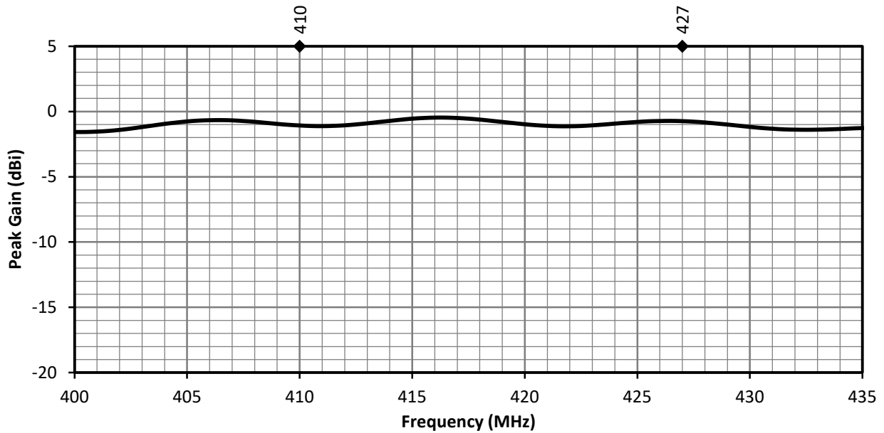
Figure 7. ANT-410-WRT Peak Gain, Free Space
