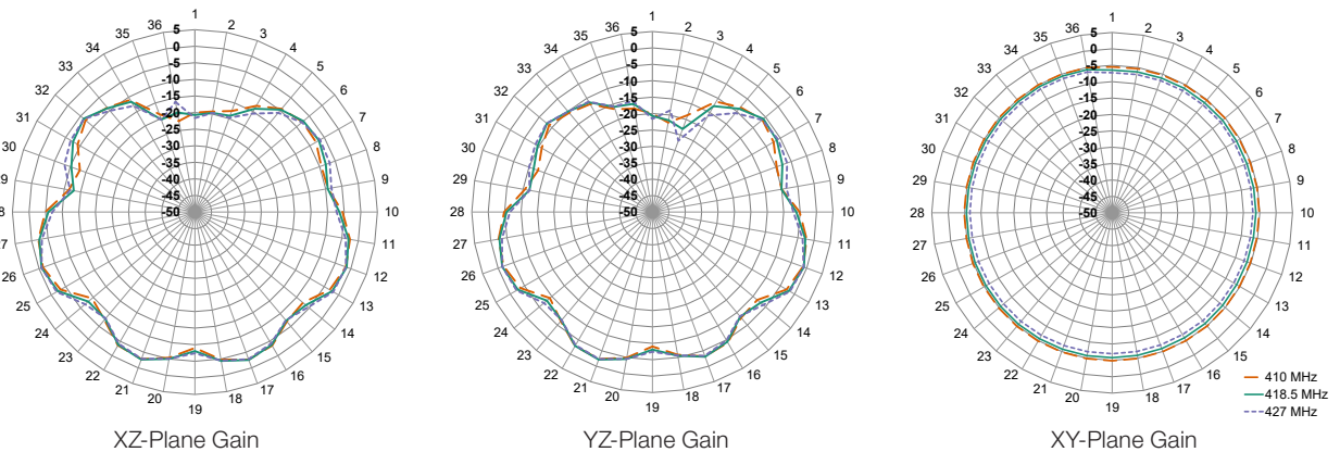
Figure 10. ANT-410-WRT Radiation Patterns, Free Space
