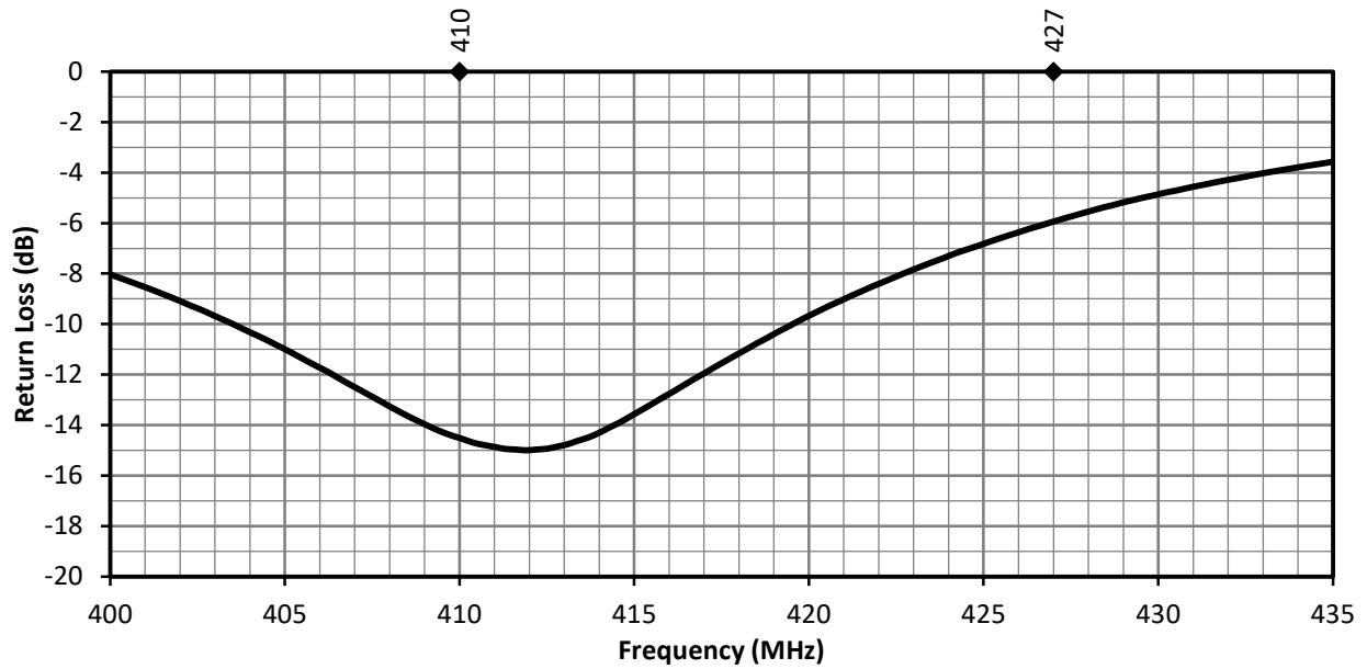
Figure 6. ANT-410-WRT Return Loss, Free Space
