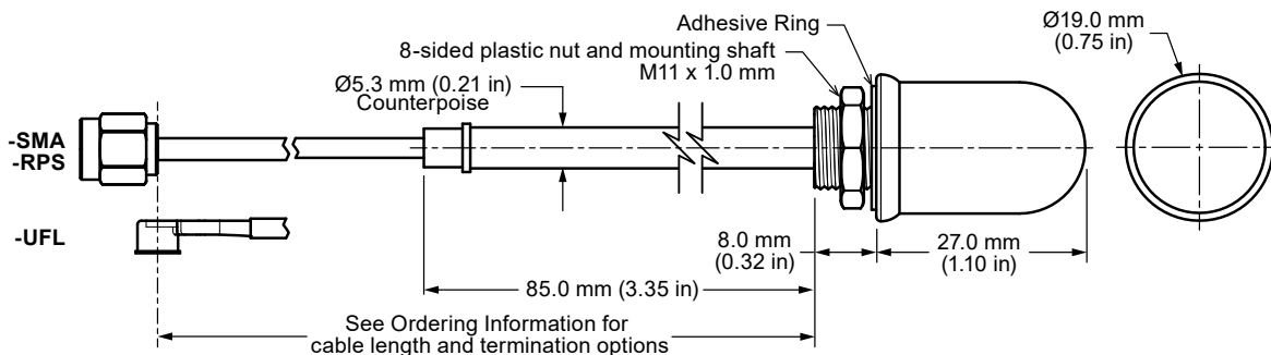
Figure 1. ANT-410-WRT-ccc Antenna Dimensions
