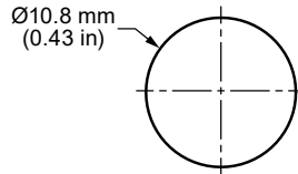
Figure 2. ANT-410-WRT Series Antenna Recommended Enclosure Mounting Dimensions
