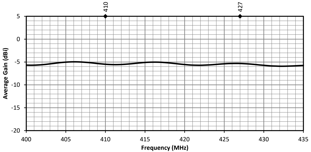
Figure 8. ANT-410-WRT Antenna Average Gain, Free Space
