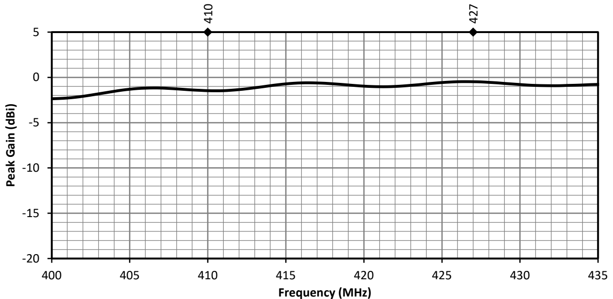
Figure 14. ANT-410-WRT Peak Gain, at Center of Ground Plane
