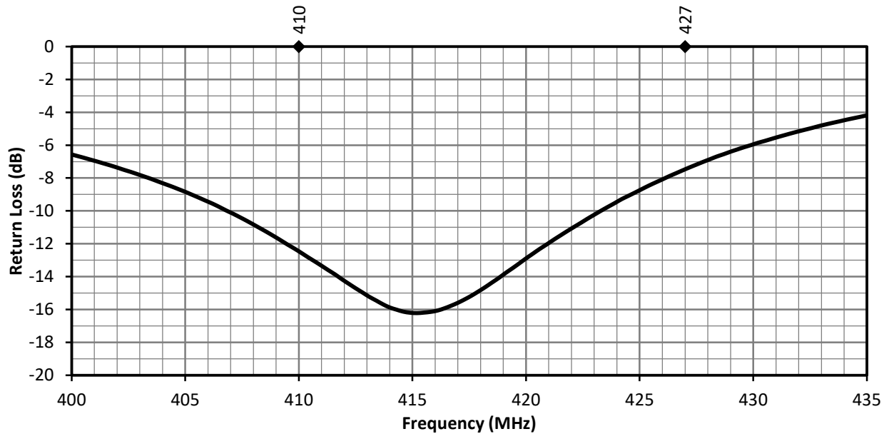
Figure 13. ANT-410-WRT Return Loss, at Center of Ground Plane
