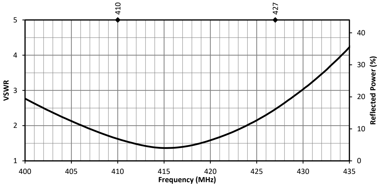
Figure 12. ANT-410-WRT VSWR, at Center of Ground Plane
