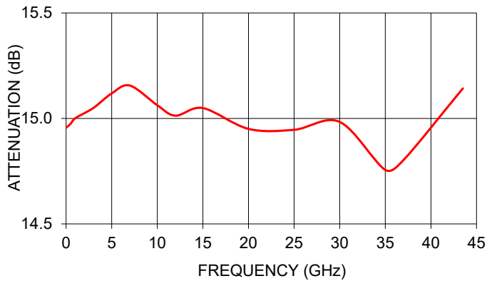
KAT-15+ ATTENUATION
