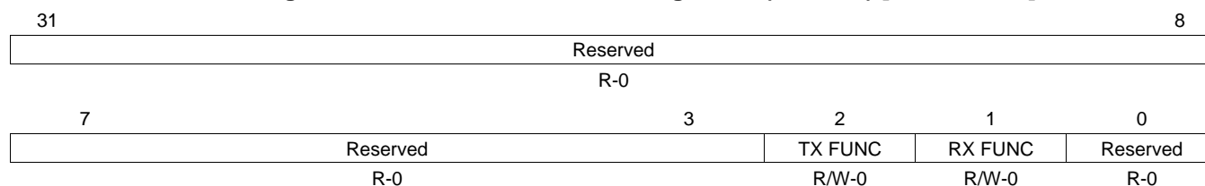
Figure 22-42. SCI Pin I/O Control Register 0 (SCIPIO0) [offset = 3Ch]
