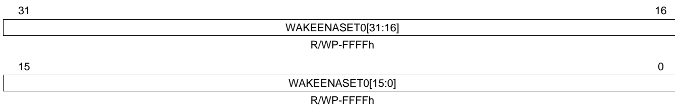
Figure 14-29. Wake-Up Enable Set Register 0 (WAKEENASET0) [offset = 50h]
