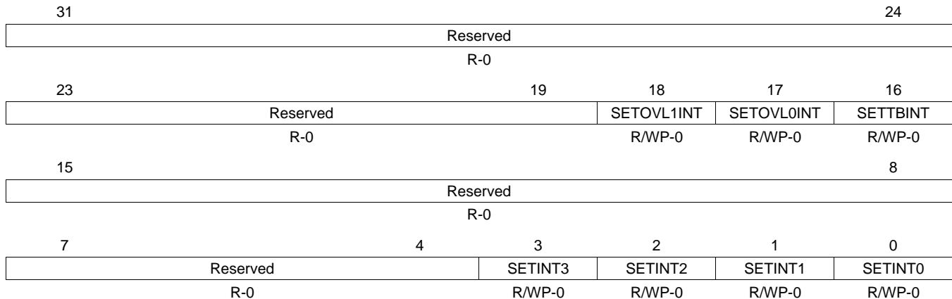
Figure 12-29. RTI Set Interrupt Control Register (RTISETINTENA) [offset = 80h]
