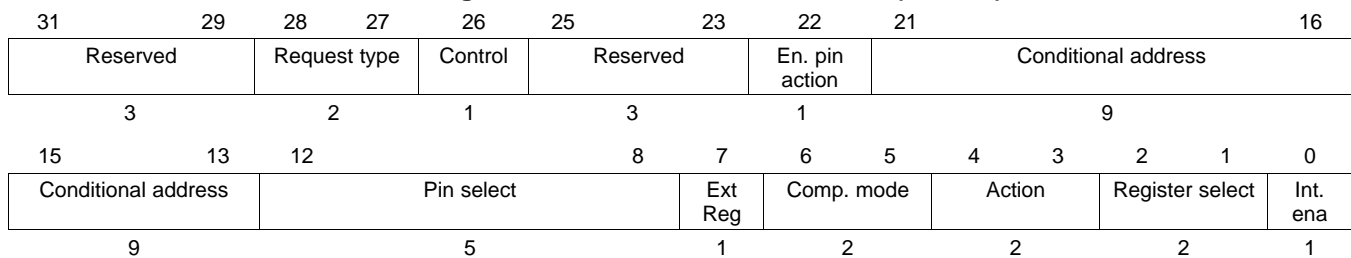
Figure 17-119. MOV64 Control Field (C31:C0)
