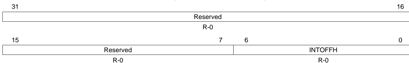
Figure 11-21. ESM Interrupt Offset High Register (ESMIOFFHR) [address = FFFF F528h]
