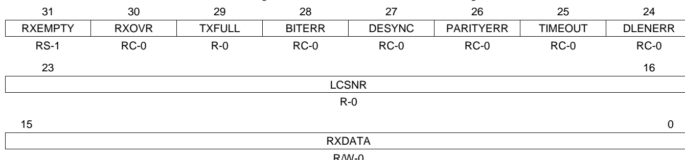
Figure 21-65. Multi-buffer RAM Receive Buffer Register (RXRAM) [offset = RAM Base + 200h-3FFh]
