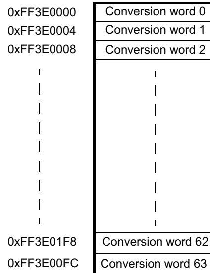
Figure 16-5. ADC Memory-Mapping
