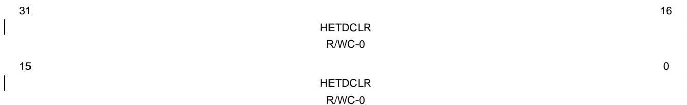
Figure 17-55. N2HET Data Clear Register (HETDCLR) [offset = 5Ch]
