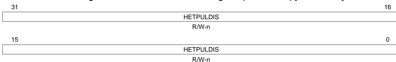
Figure 17-57. N2HET Pull Disable Register (HETPULDIS) [offset = 64h]
