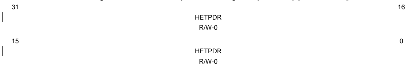
Figure 17-56. N2HET Open Drain Register (HETPDR) [offset = 60h]
