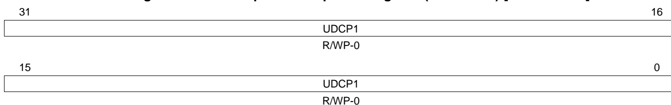
Figure 12-24. RTI Update Compare 1 Register (RTIUDCP1) [offset = 5Ch]
