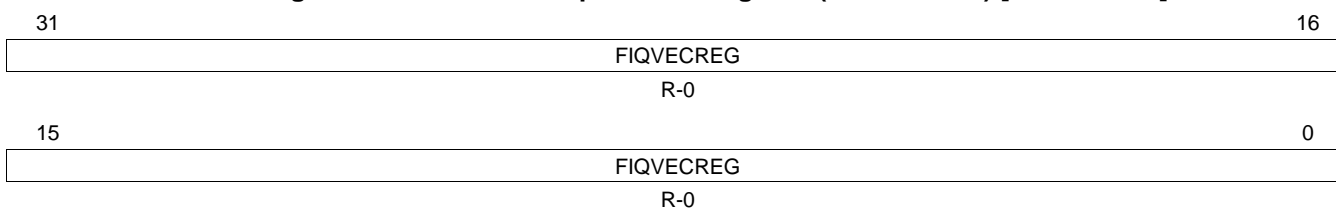
Figure 14-36. IRQ Interrupt Vector Register (FIQVECREG) [offset = 74h]
