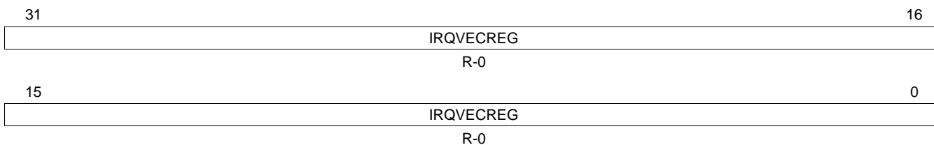
Figure 14-35. IRQ Interrupt Vector Register (IRQVECREG) [offset = 70h]
