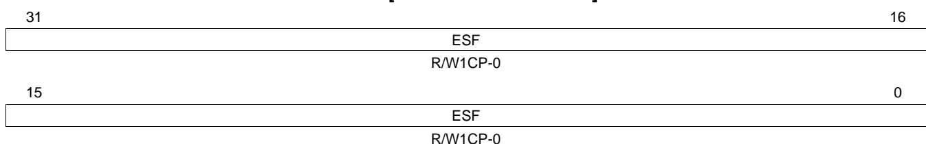
Figure 11-18. ESM Status Register 2 (ESMSR2) [address = FFFF F51Ch]
