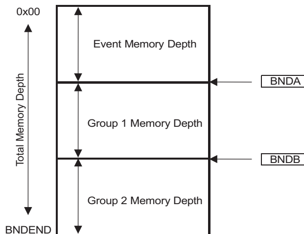
Figure 16-2. FIFO Implementation
