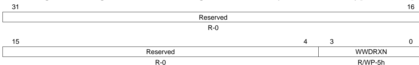
Figure 12-37. Digital Windowed Watchdog Reaction Control (RTIWWDRXNCTRL) [offset = A4h]
