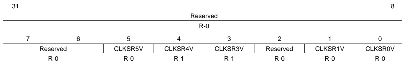
Figure 2-22. Clock Source Valid Status Register (CSVSTAT) (offset = 54h)
