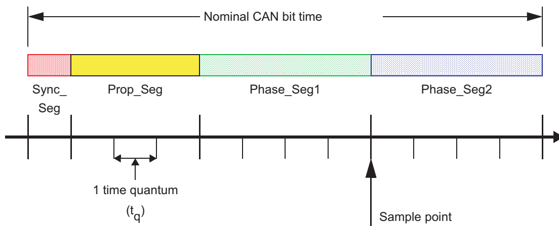
Figure 20-2. Bit Timing
