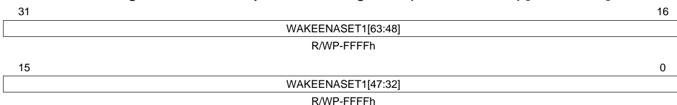
Figure 14-30. Wake-Up Enable Set Register 1 (WAKEENASET1) [offset = 54h]
