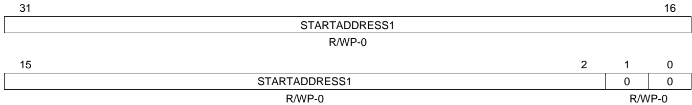
Figure 18-31. Memory Protection 1 Start Address Register (HTU MP1S) [offset = 4Ch]
