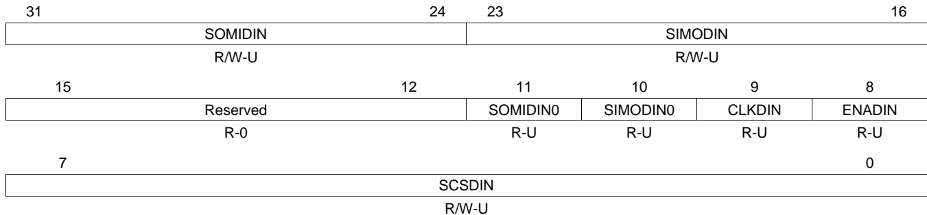
Figure 21-24. SPI Pin Control Register 2 (SPIPC2) [offset = 1Ch]
