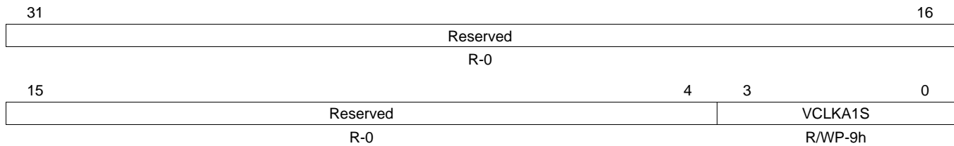
Figure 2-20. Peripheral Asynchronous Clock Source Register (VCLKASRC) (offset = 4Ch)
