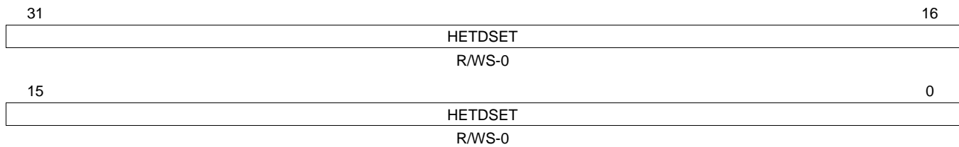
Figure 17-54. N2HET Data Set Register (HETDSET) [offset = 58h]
