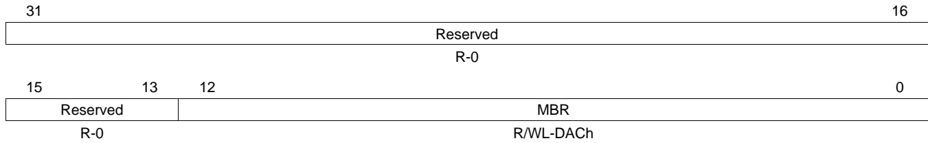
Figure 22-58. Maximum Baud Rate Selection Register (MBRS) [offset = 7Ch]
