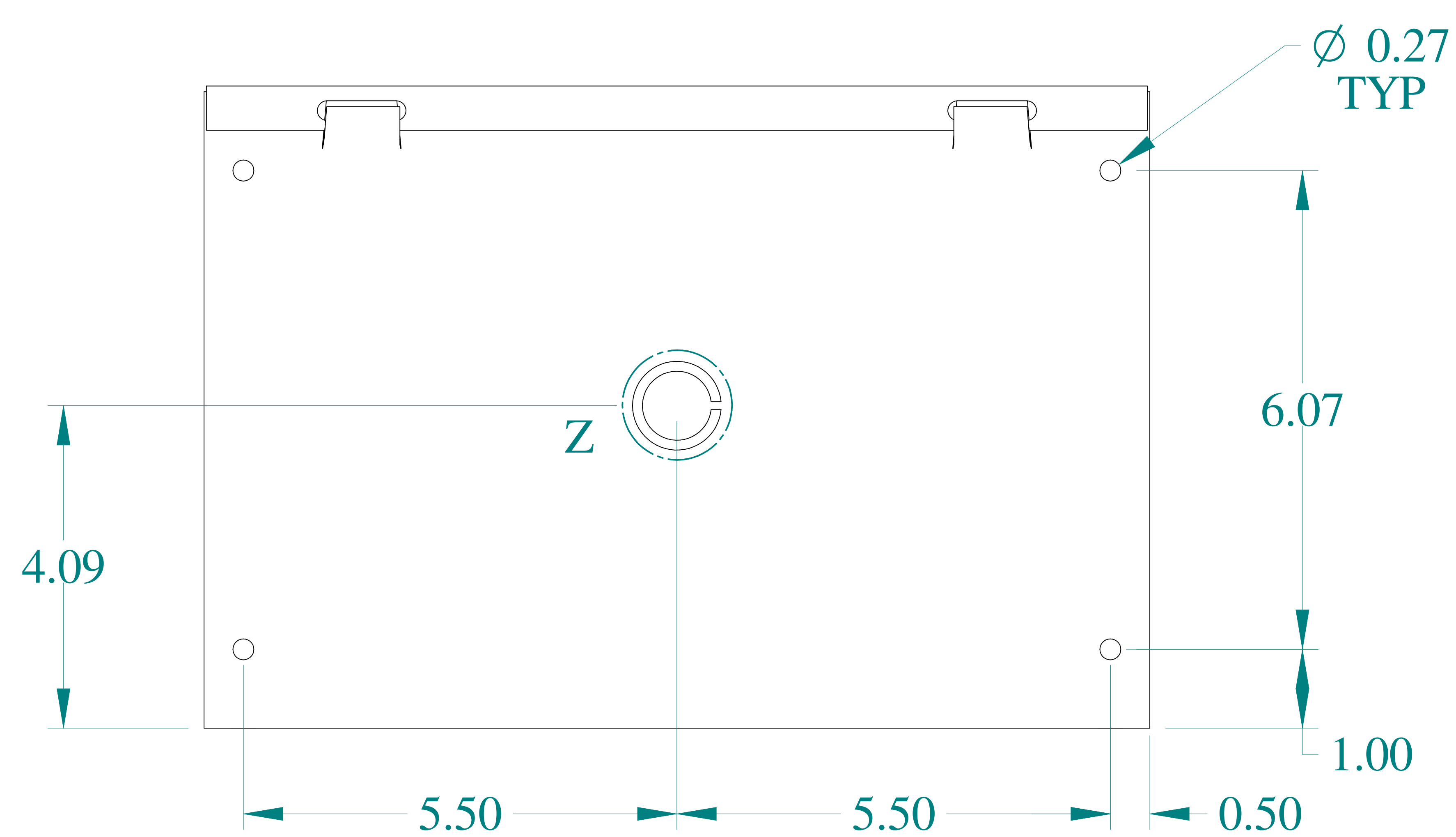
SIDE VIEW
