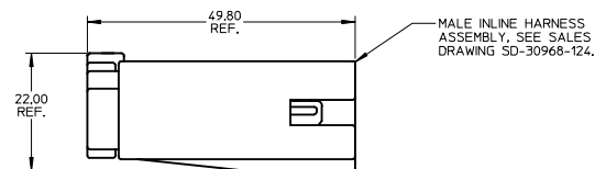
MATED VIEW
