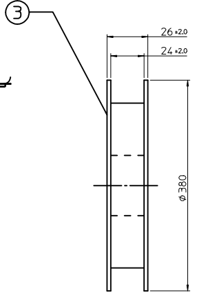
PLASTIC BOBBIN
