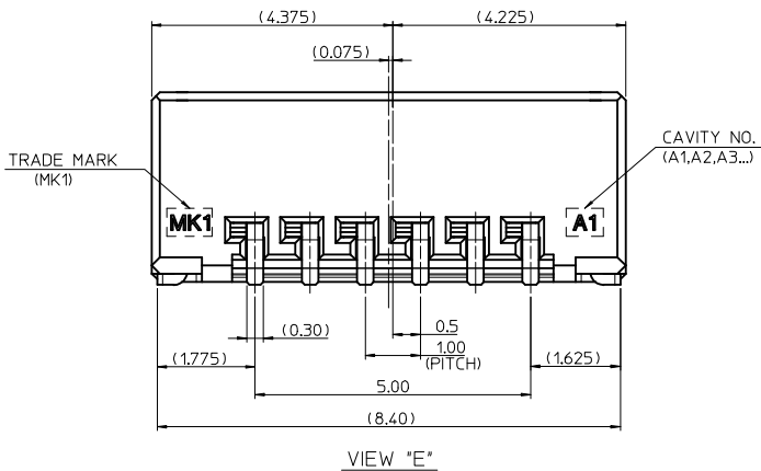
VIEW "E"
