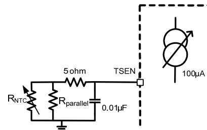
Figure 45: Temperature Sense NTC Network
