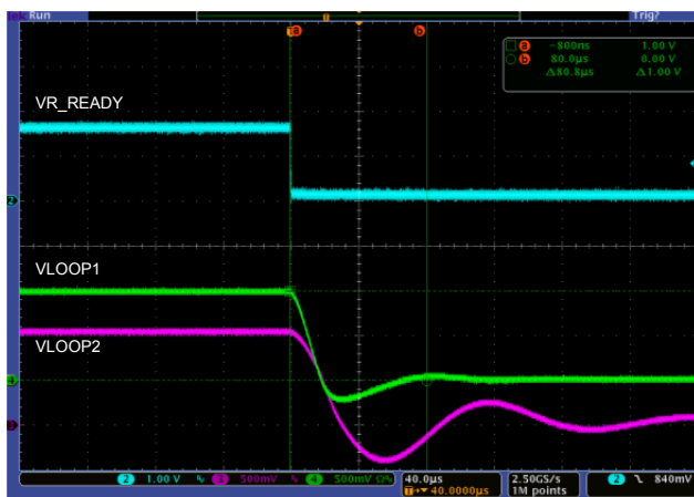
Figure 42: OVP - MOSFET latched on
