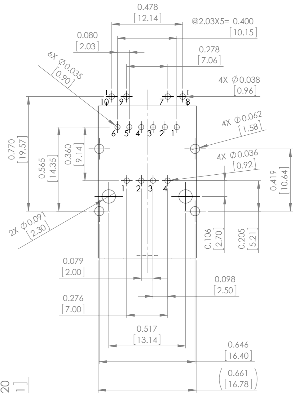
PC BOARD LAYOUT COMPONENT SIDE SHOWN
