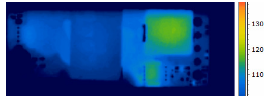
Thermal Image of module @ 48Vin, 200LFM & 70C
