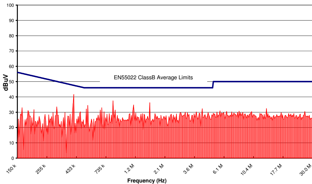
Figure 18. CPE6B36 Conducted Emissions using above specified input filter, Vin = 48V, Full Resistive Load
