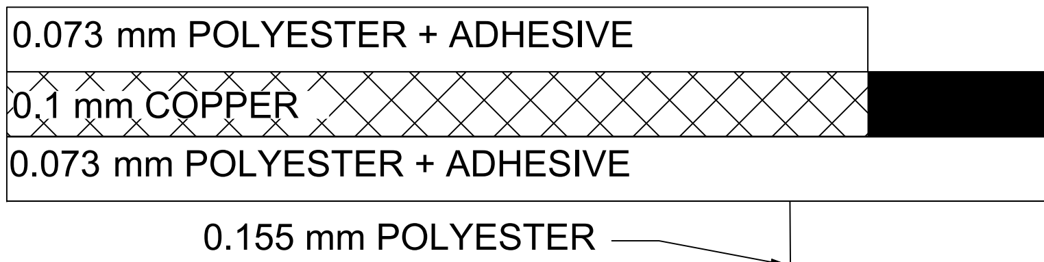
CROSS-SECTION
