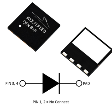
Package Types: QFN 8x8 Marking: C6D10065Q
