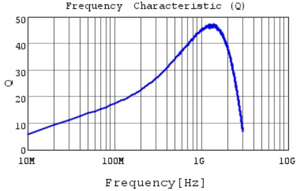
LQG15WZ19NJ02 Q
