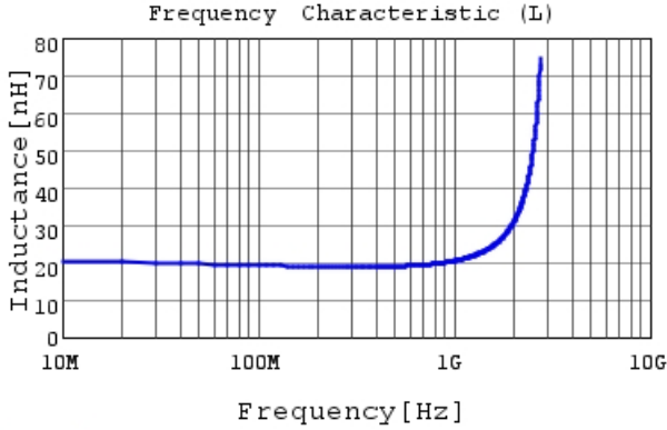
LQG15WZ19NJ02 L
