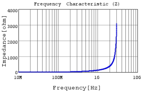
LQG15WZ19NJ02 |Z|
