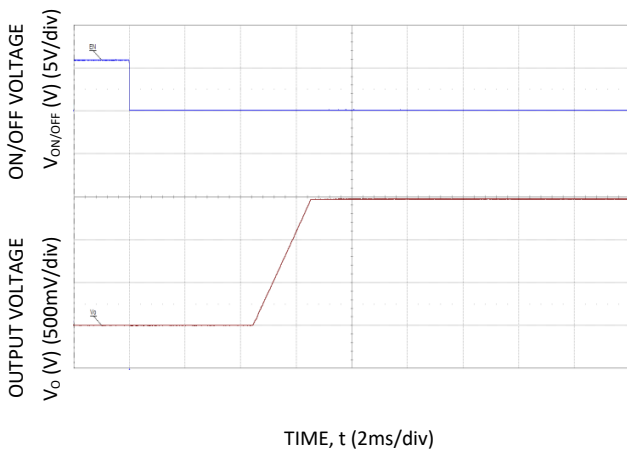
Figure 29. Typical Start-up Using On/Off Voltage ( V_{in} = 12\text{V} , I_o = I_{o,max} .)
