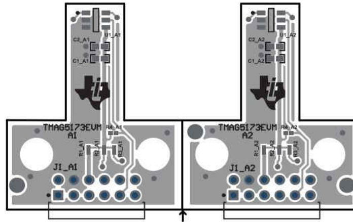
Figure 6-11. TMAP5173EVM Top View
