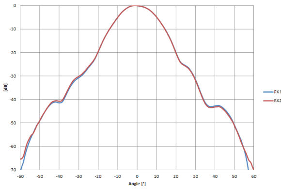
IVQ-3005 system-pattern (AZIMUTH)
