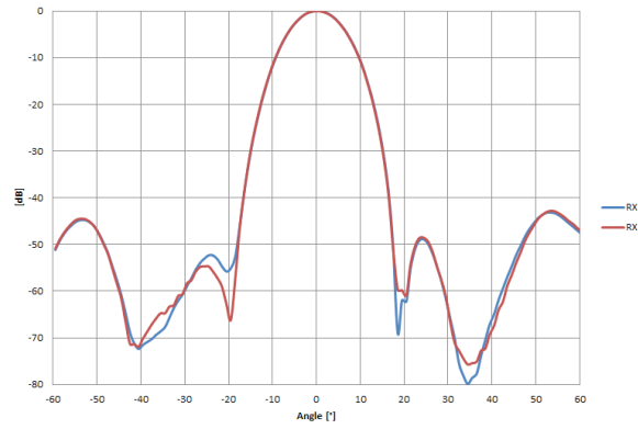
IVQ-3005 system-pattern (ELEVATION)
