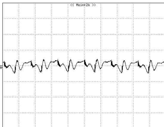
Figure 12: Output voltage ripple at nominal input voltage ( v_{in}=48\text{v} ) and rated load current ( I_o=10\text{A} ) (50 mV/div, 1us/div). Load capacitance: 1\ \mu\text{F} ceramic capacitor and 100\ \mu\text{F} tantalum capacitor. Bandwidth: 20 MHz. Scope measurements should be made using a BNC cable (length shorter than 20 inches). Position the load between 51 mm to 76 mm (2 inches to 3 inches) from the module
