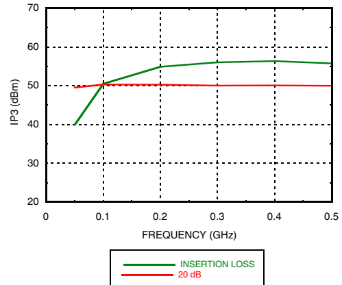
Input IP3 vs. Frequency (Low Frequency Detail)
