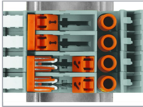
Switch positions
