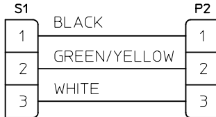
WIRING DIAGRAM
