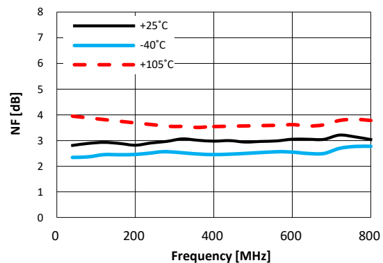
Figure 15. Noise Figure vs. Frequency Over Temperature (Max Gain State)
