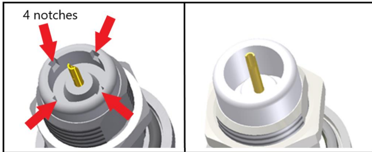
Termination view without potting for clarity
